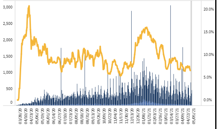
Number of Testing Encounters, Number of Positive Testing Encounters, and Percent Positivity** by Lab Report Date - Crater, PCR Only
